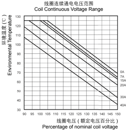
允许最大负载范围 (23°C) Max.imum allowable load range
